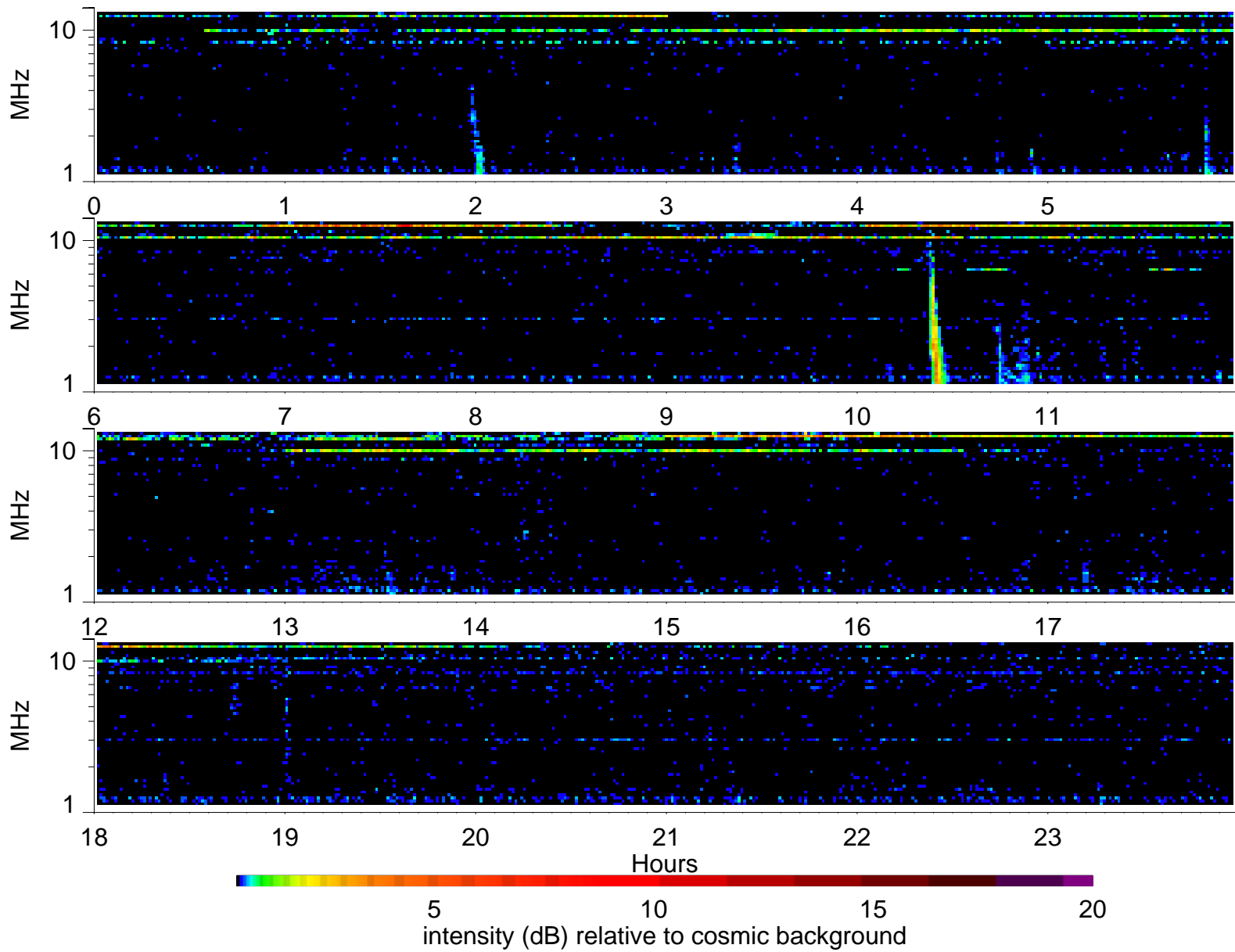
Wind Waves RAD2 receiver: 2005/7/4
