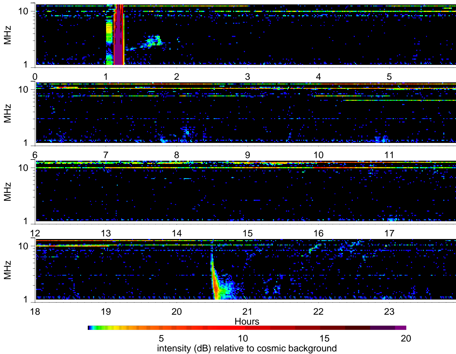
Wind Waves RAD2 receiver: 2005/6/25
