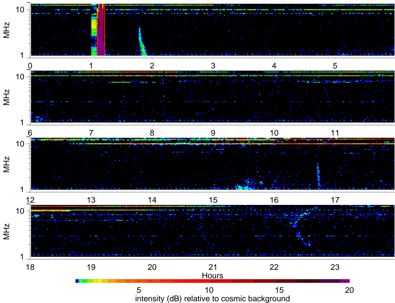
Wind Waves RAD2 receiver: 2005/6/23
