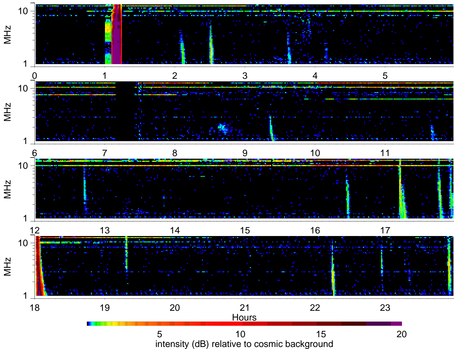
Wind Waves RAD2 receiver: 2005/6/21
