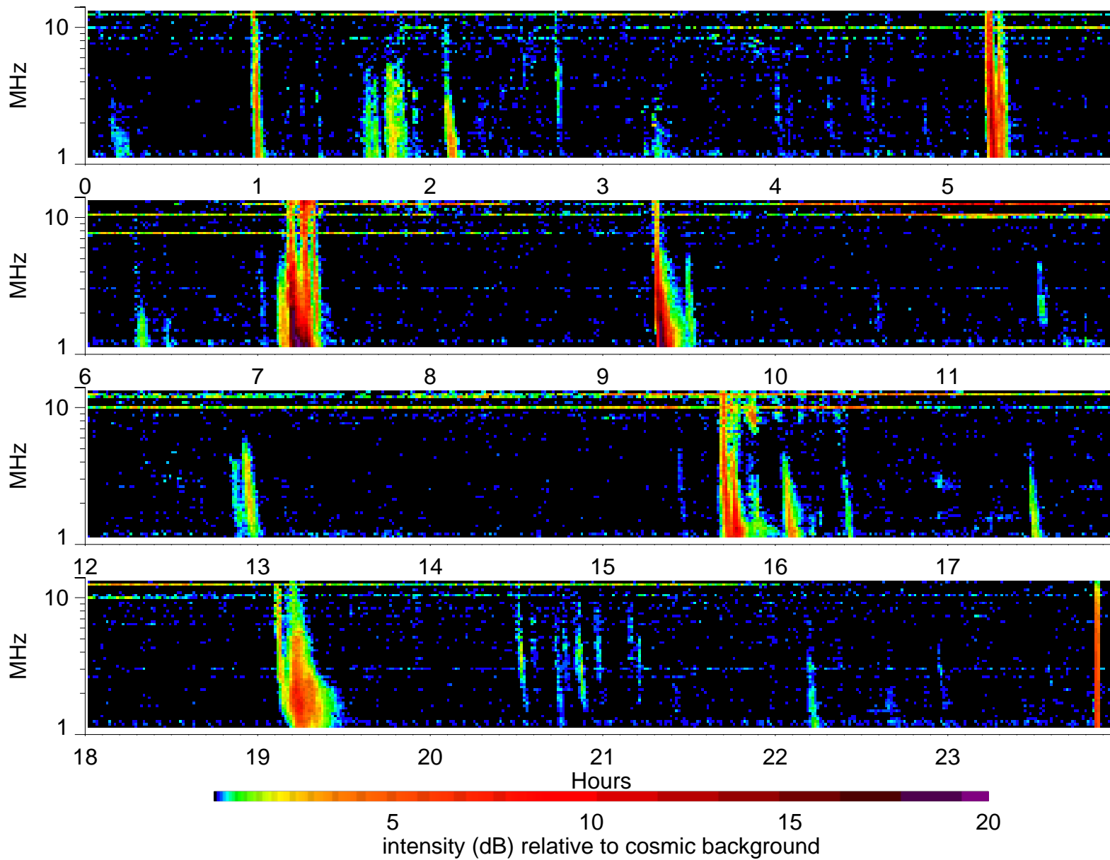
Wind Waves RAD2 receiver: 2005/6/14
