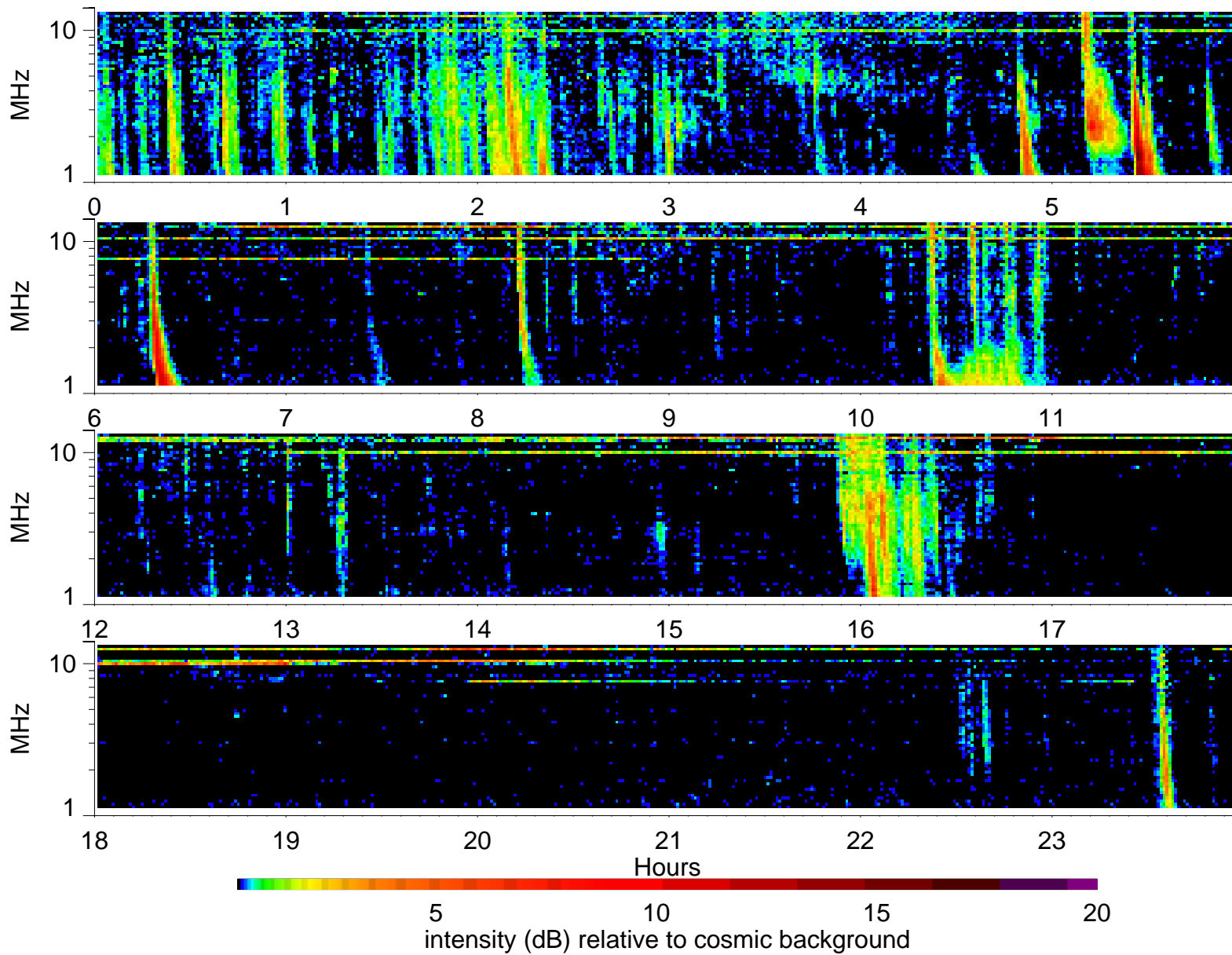
Wind Waves RAD2 receiver: 2005/6/12
