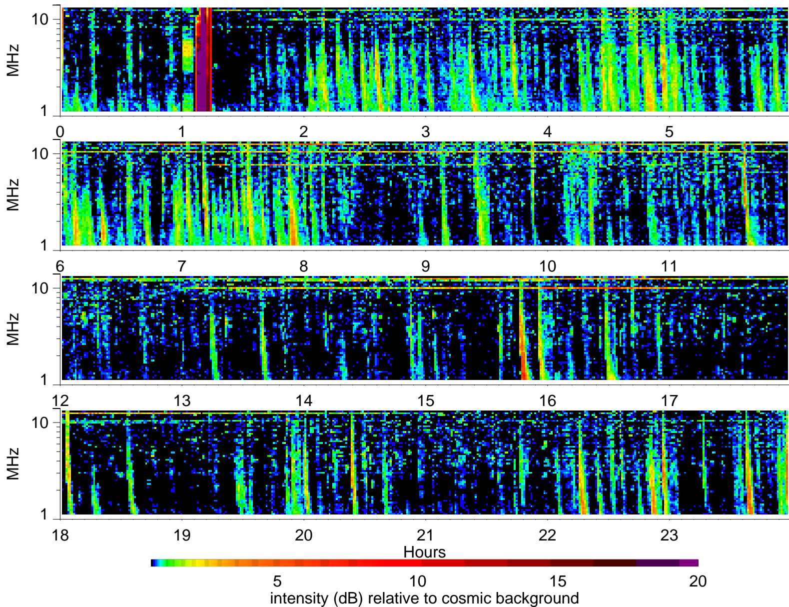
Wind Waves RAD2 receiver: 2005/6/11
