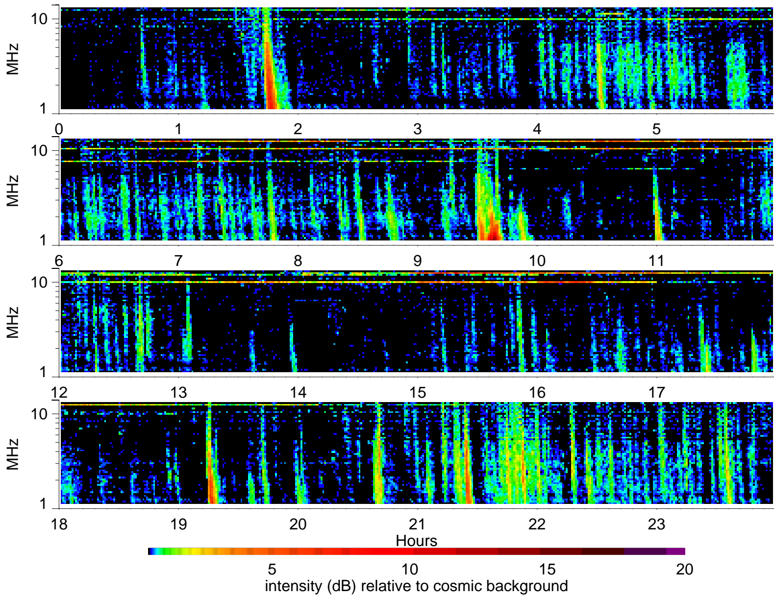
Wind Waves RAD2 receiver: 2005/6/8
