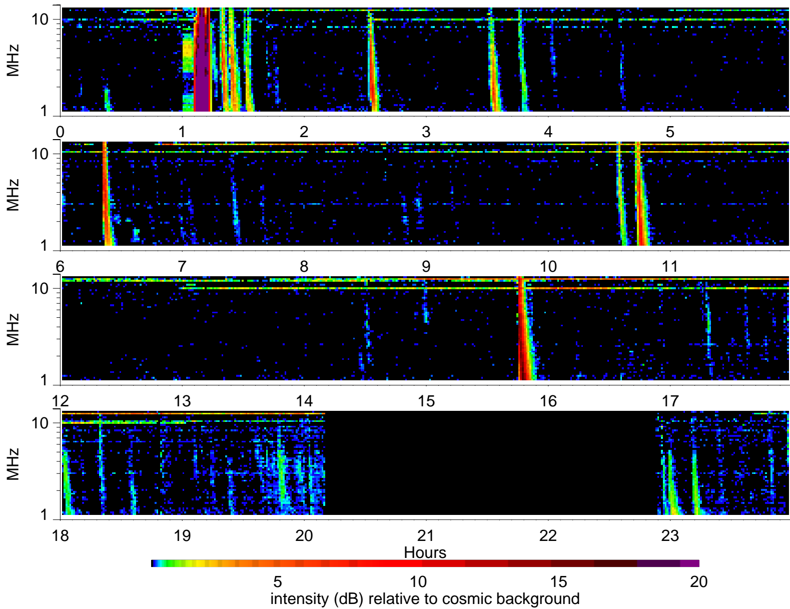
Wind Waves RAD2 receiver: 2005/6/7
