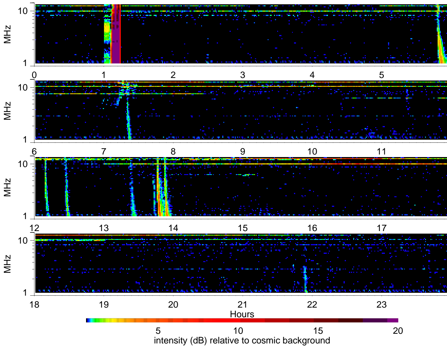
Wind Waves RAD2 receiver: 2005/6/5
