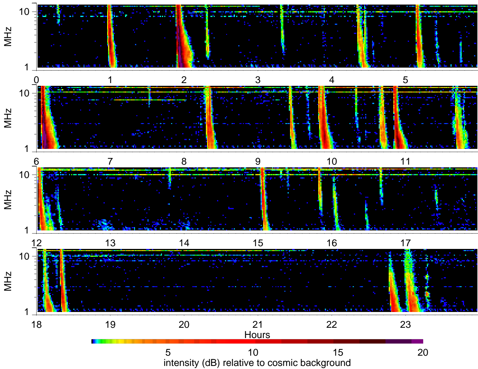
Wind Waves RAD2 receiver: 2005/6/2
