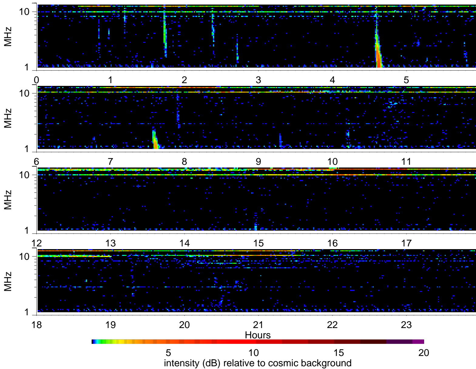
Wind Waves RAD2 receiver: 2005/5/29
