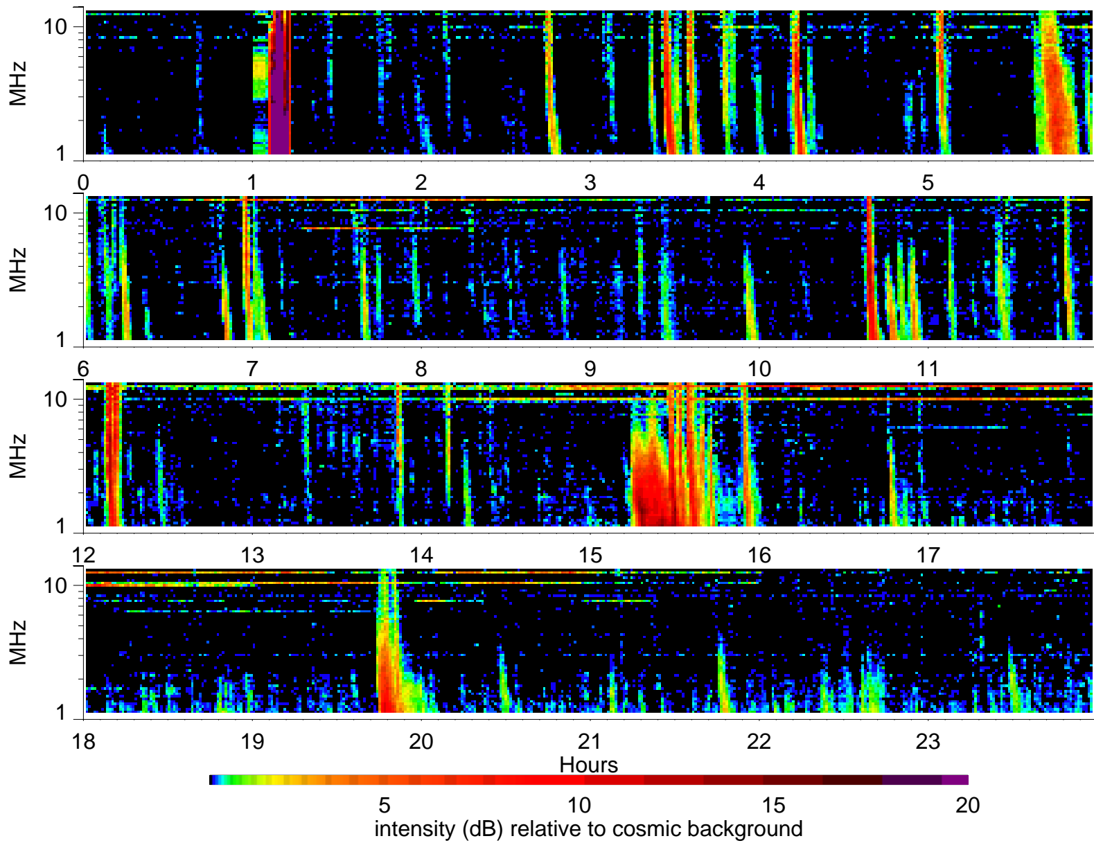
Wind Waves RAD2 receiver: 2005/5/8
