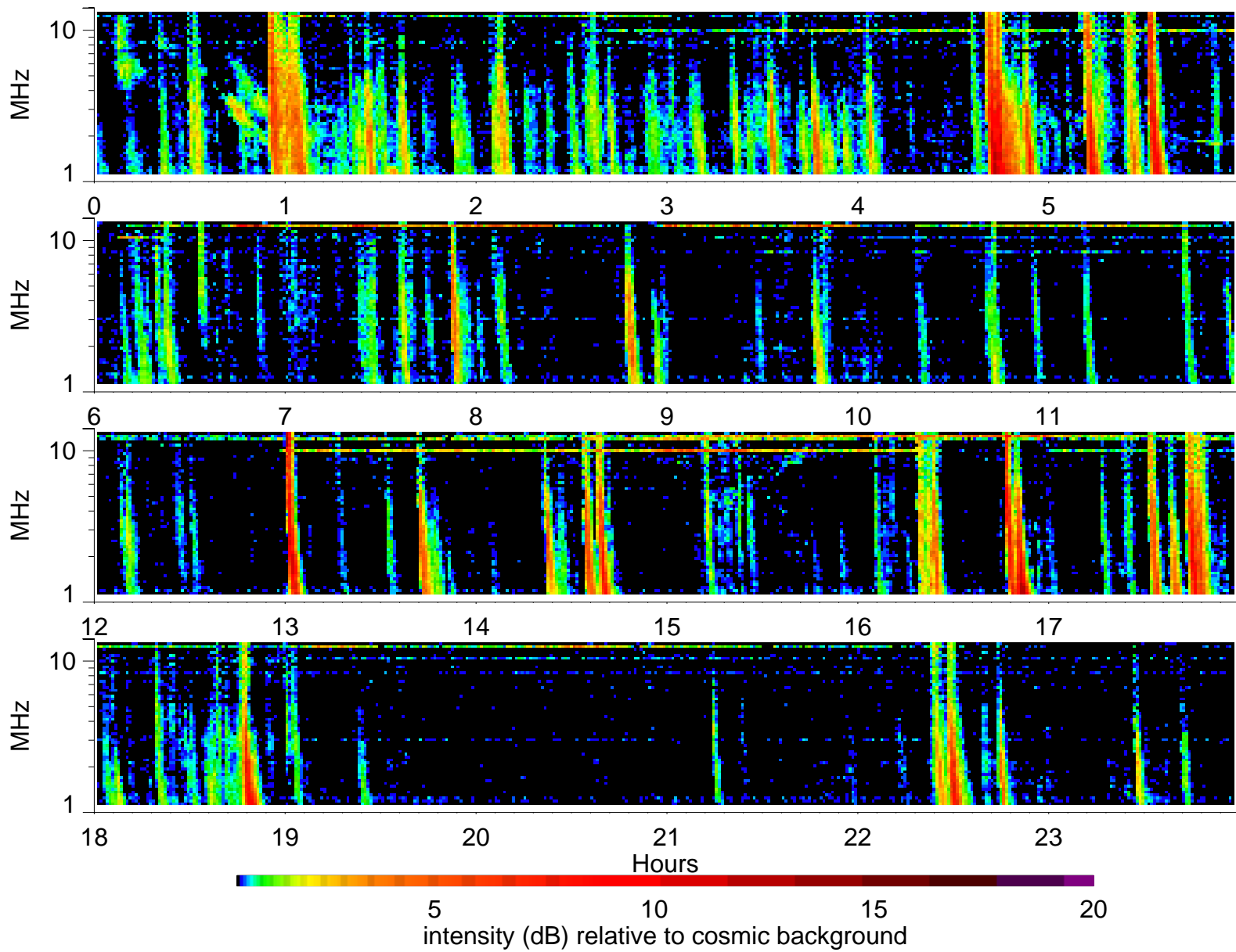
Wind Waves RAD2 receiver: 2005/5/3
