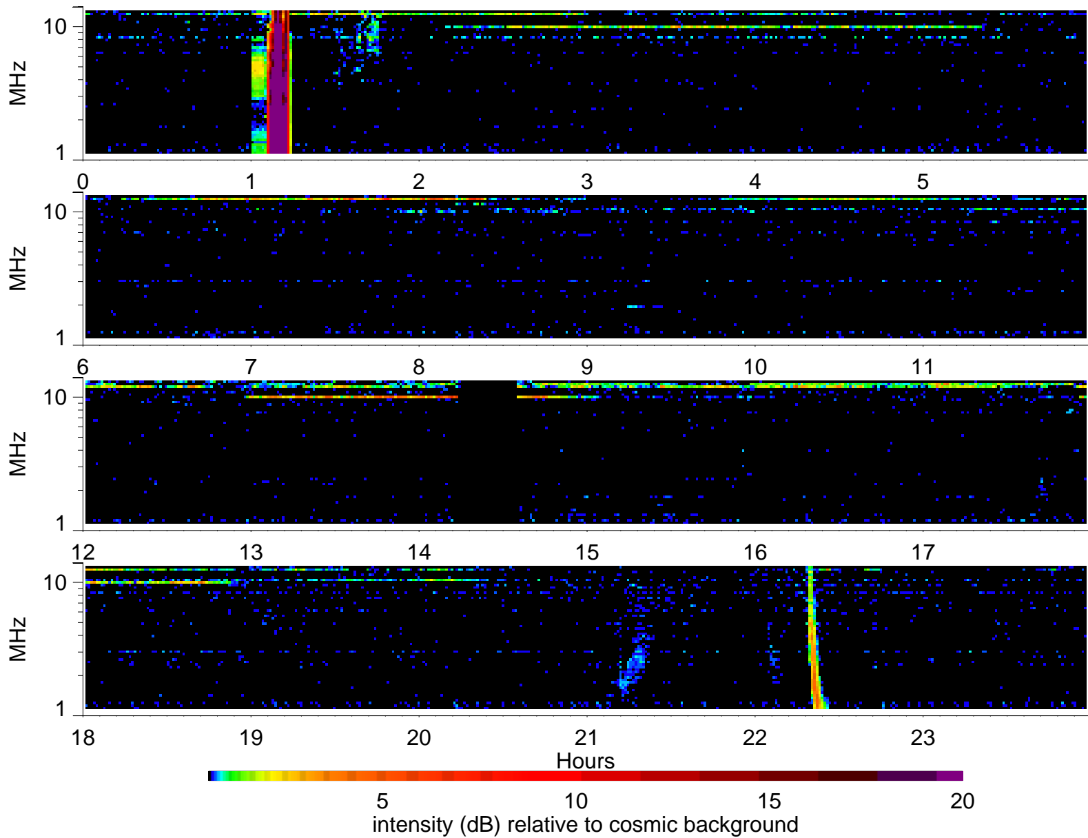
Wind Waves RAD2 receiver: 2005/4/22
