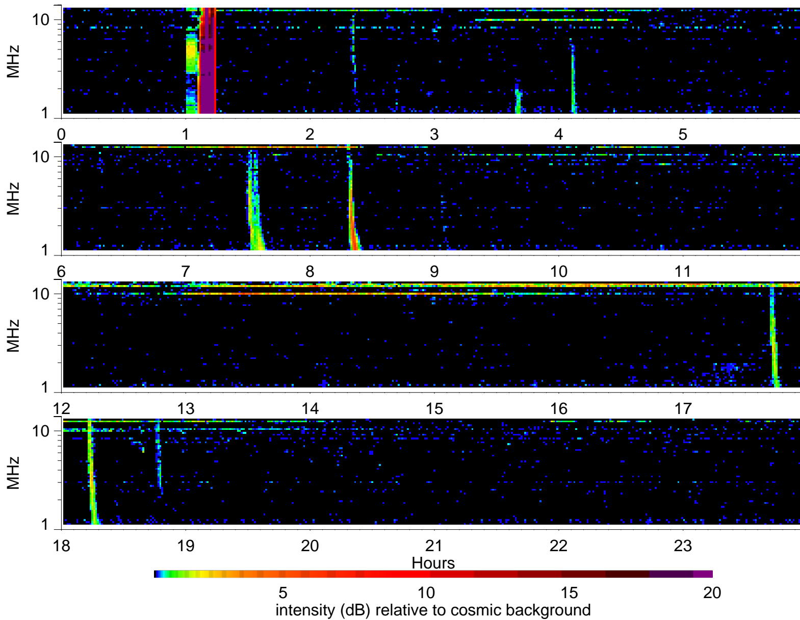
Wind Waves RAD2 receiver: 2005/4/20
