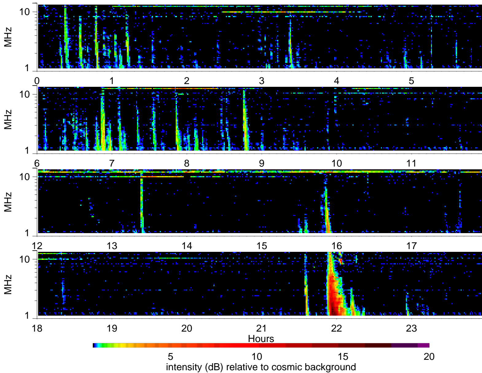
Wind Waves RAD2 receiver: 2005/4/19
