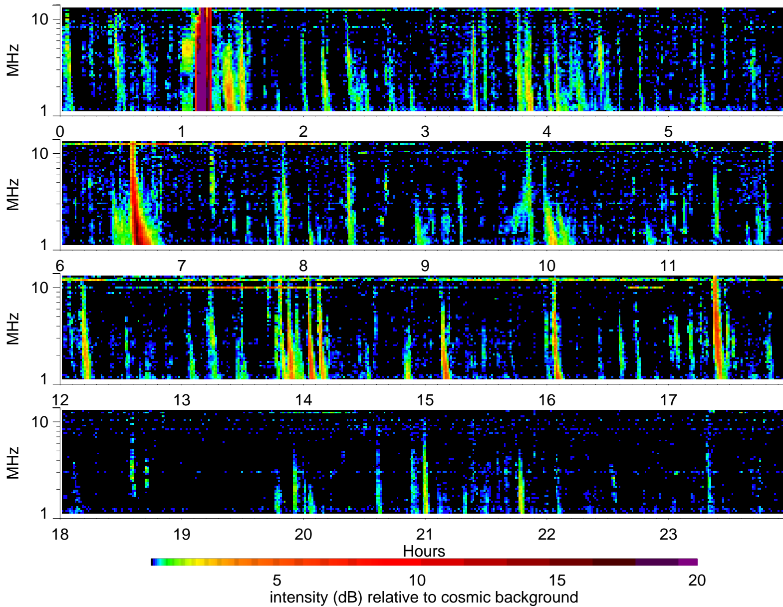
Wind Waves RAD2 receiver: 2005/4/18
