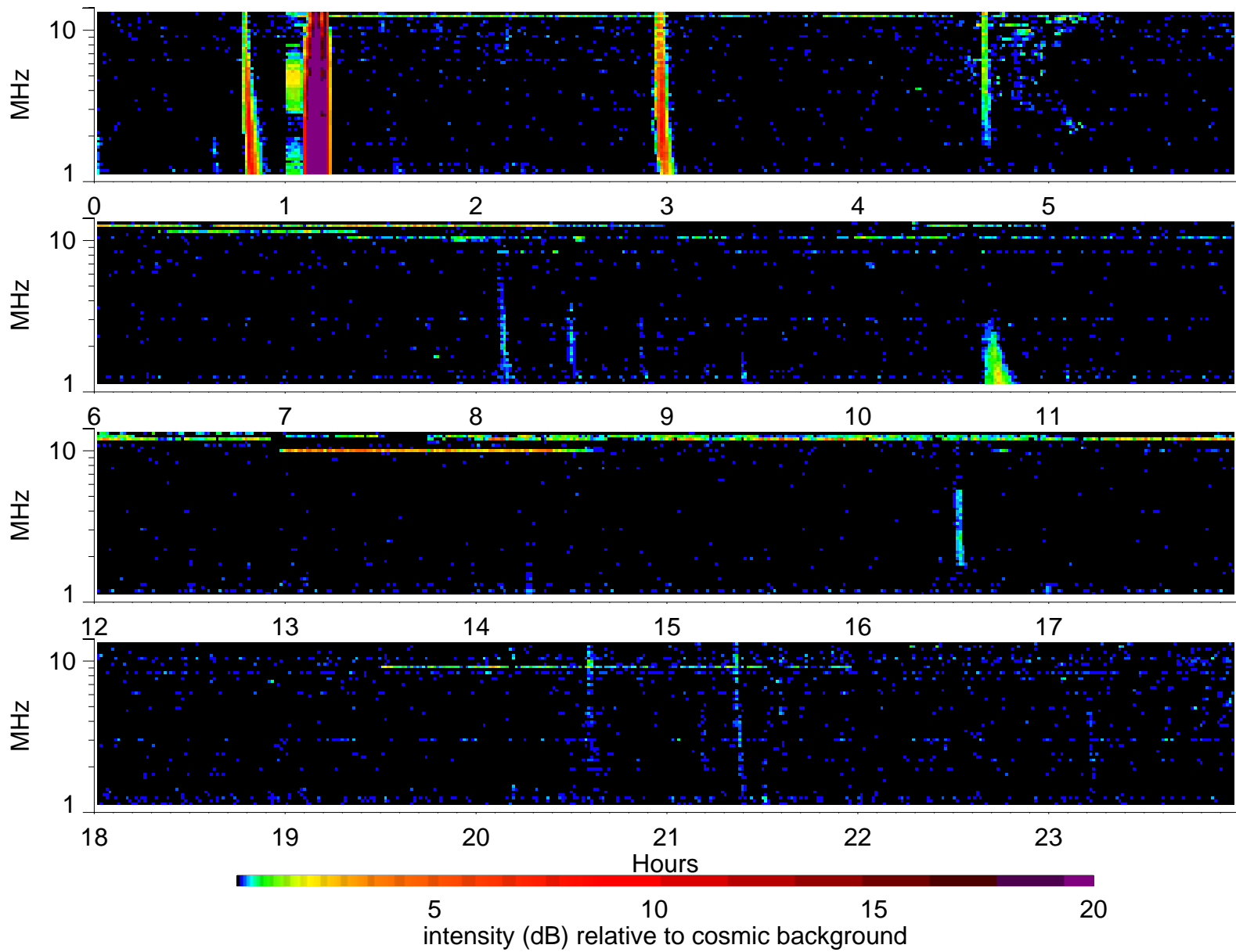
Wind Waves RAD2 receiver: 2005/4/14
