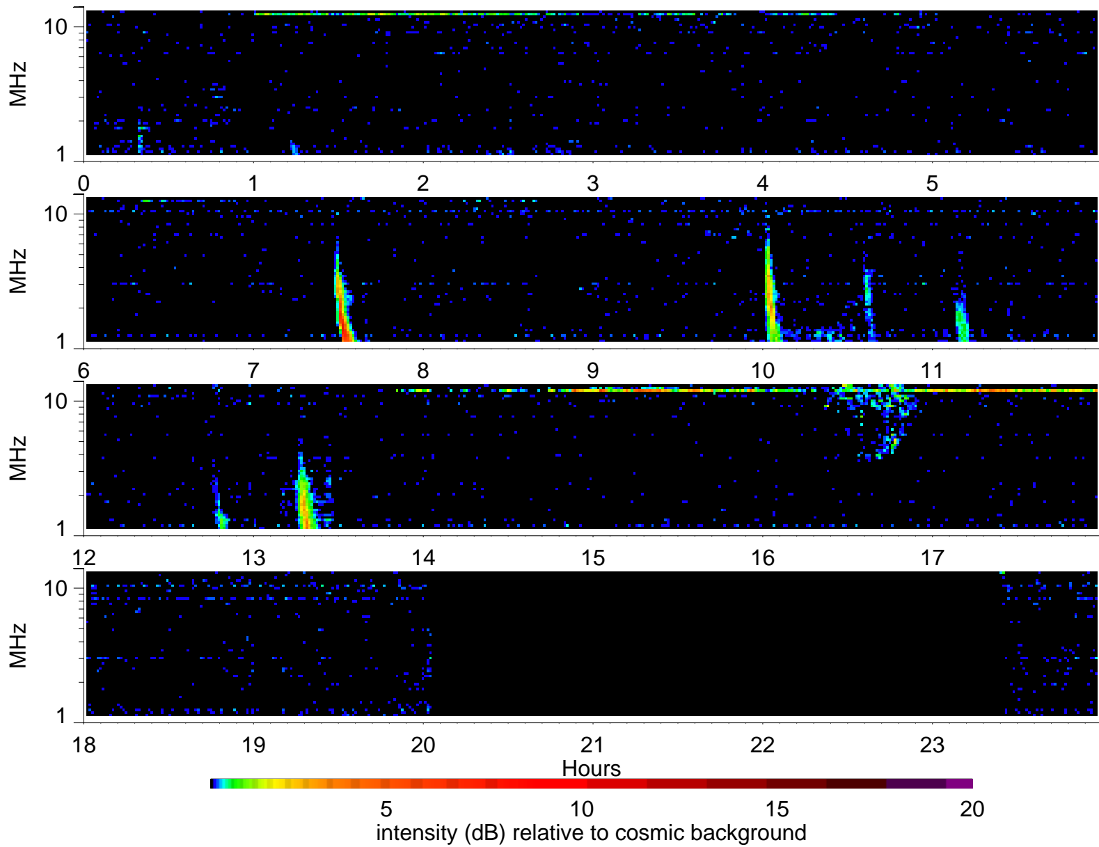
Wind Waves RAD2 receiver: 2005/4/9
