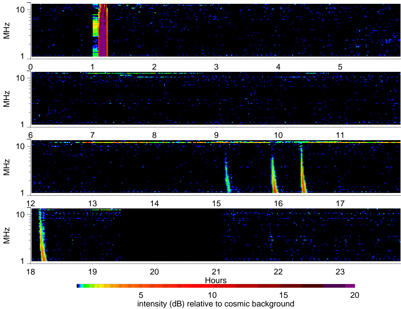
Wind Waves RAD2 receiver: 2005/4/6
