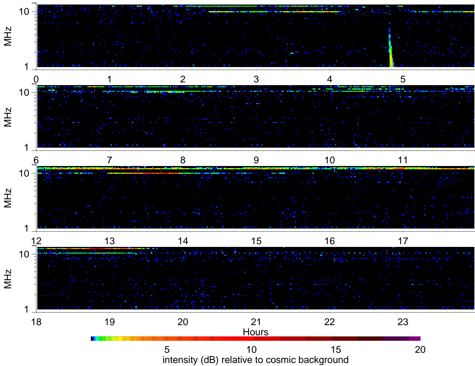
Wind Waves RAD2 receiver: 2005/4/5
