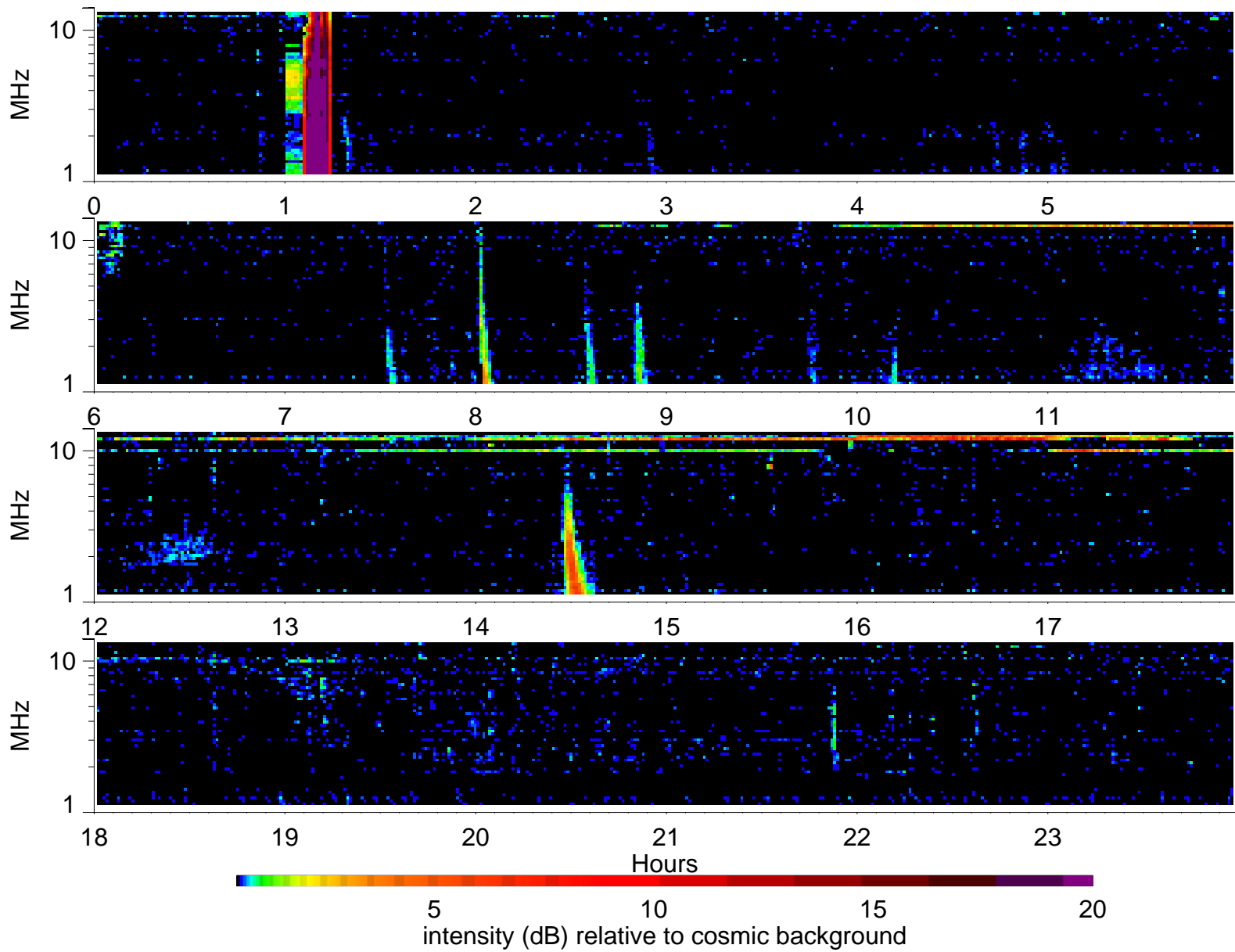
Wind Waves RAD2 receiver: 2005/3/21
