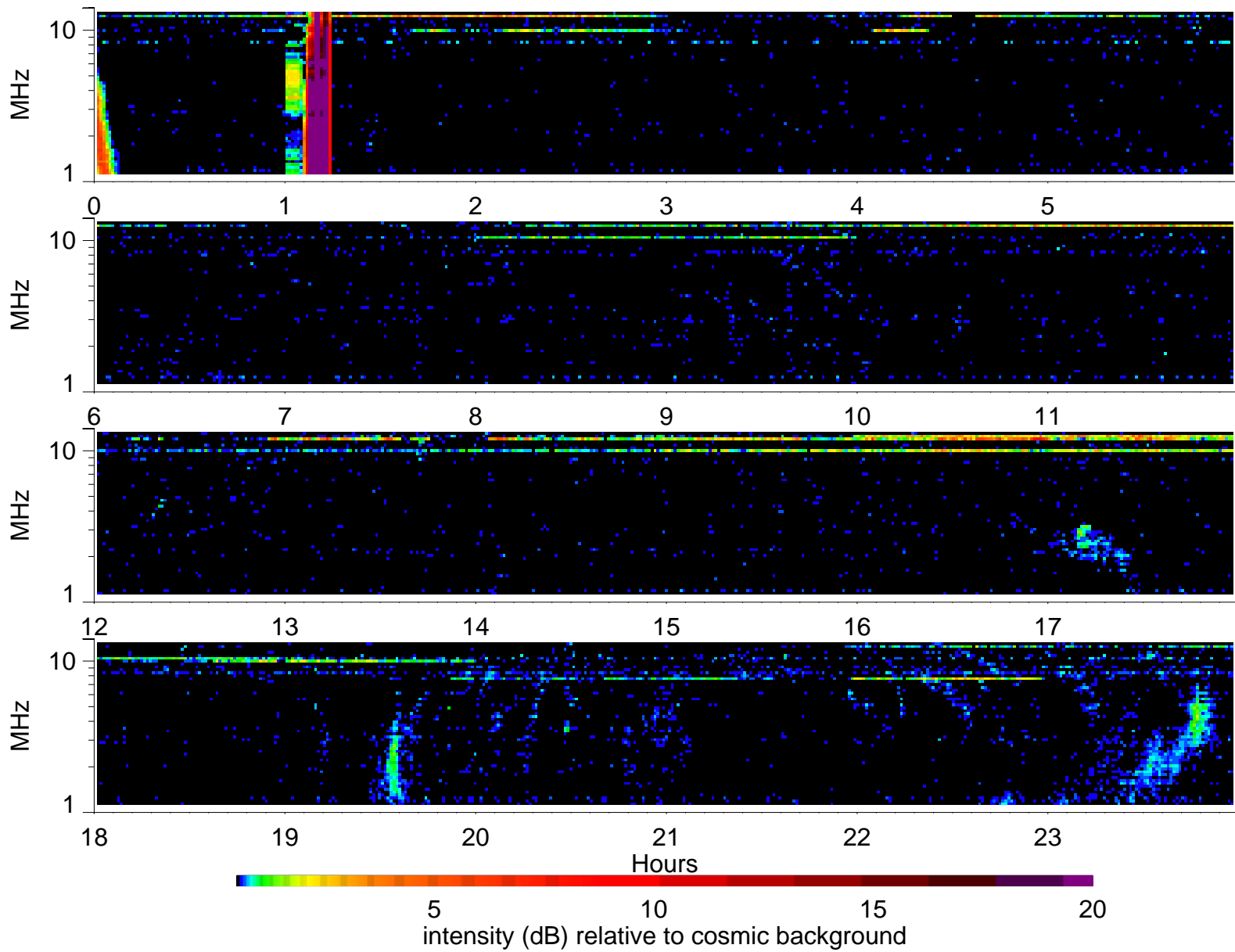
Wind Waves RAD2 receiver: 2005/3/5
