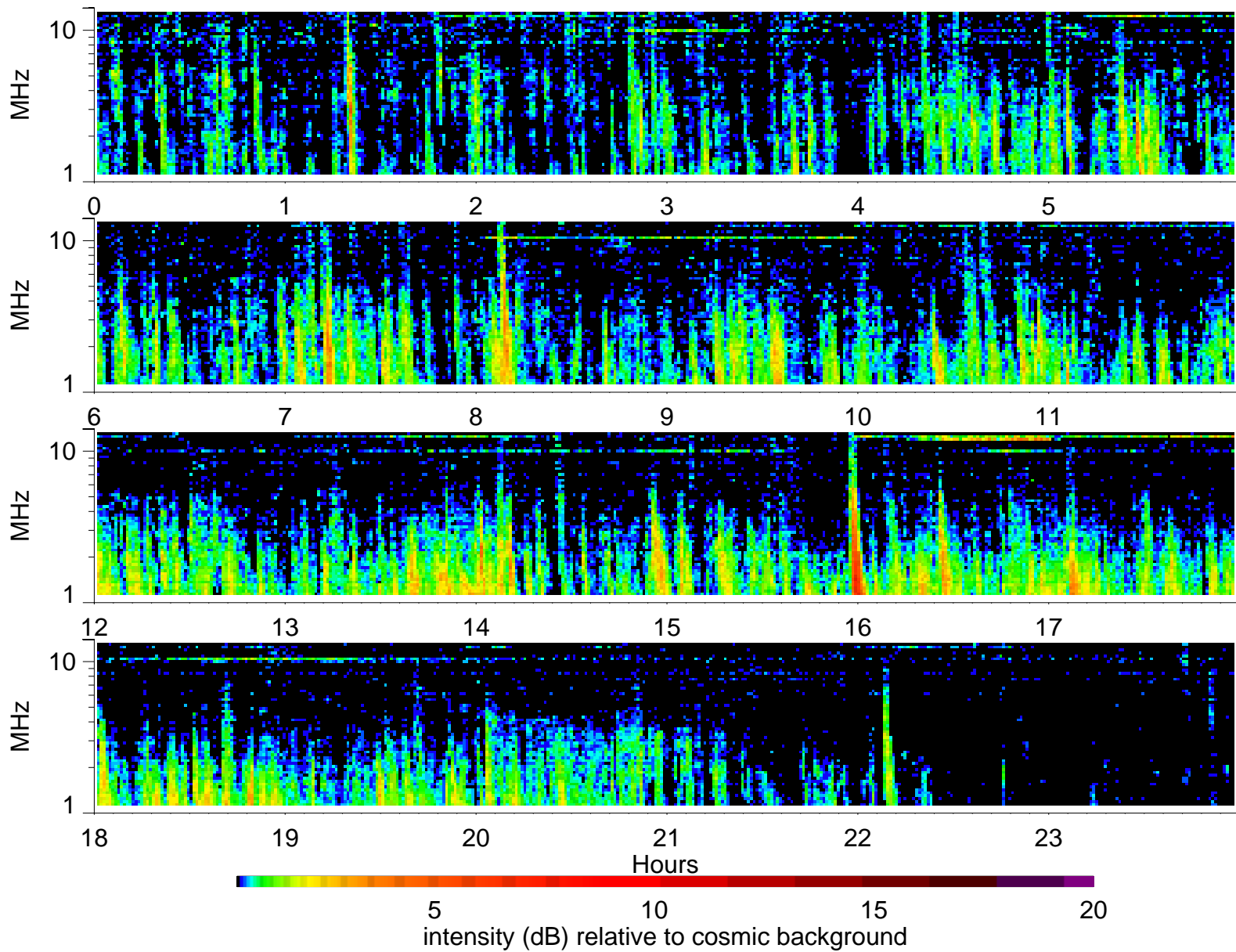
Wind Waves RAD2 receiver: 2005/2/18
