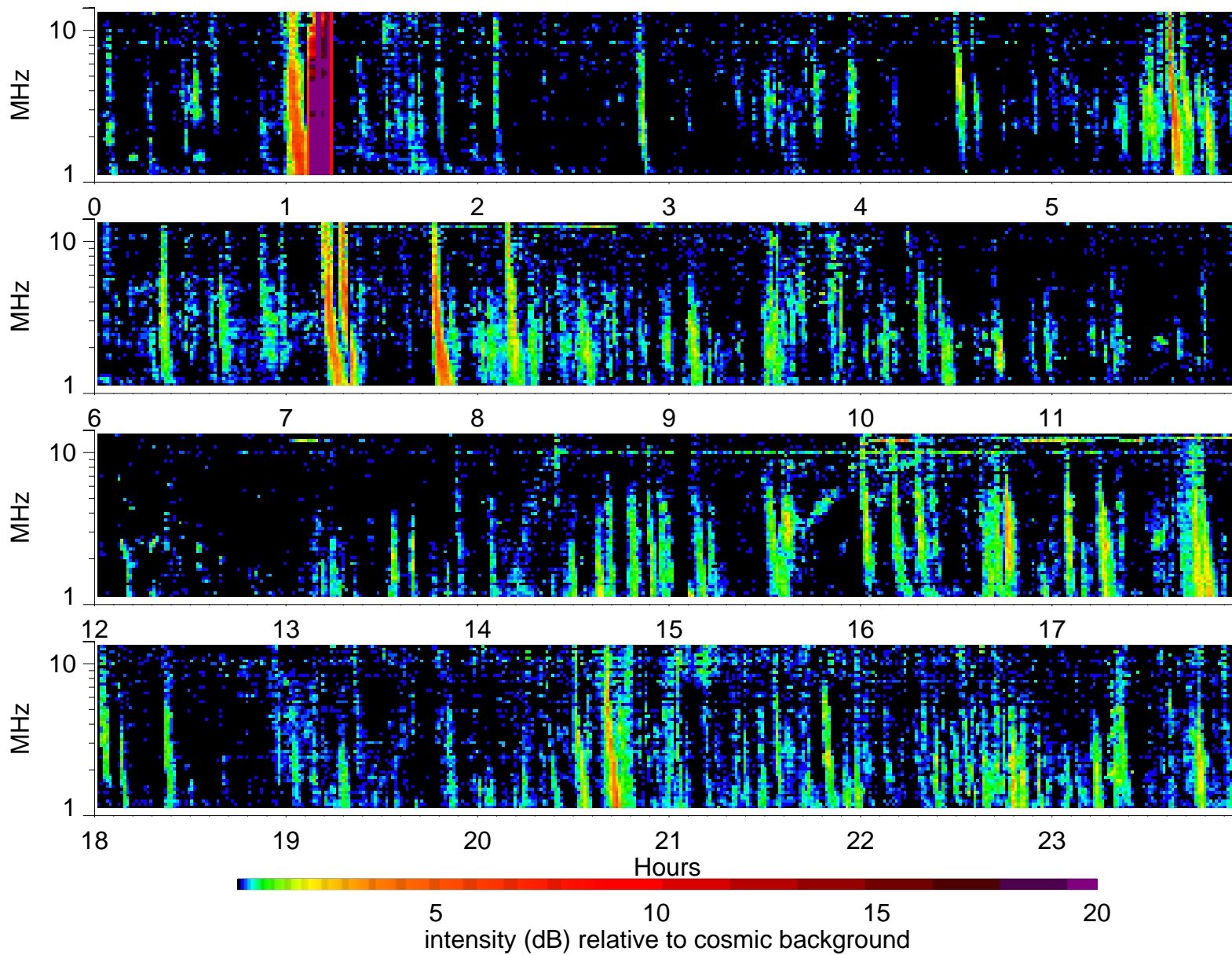
Wind Waves RAD2 receiver: 2005/2/17
