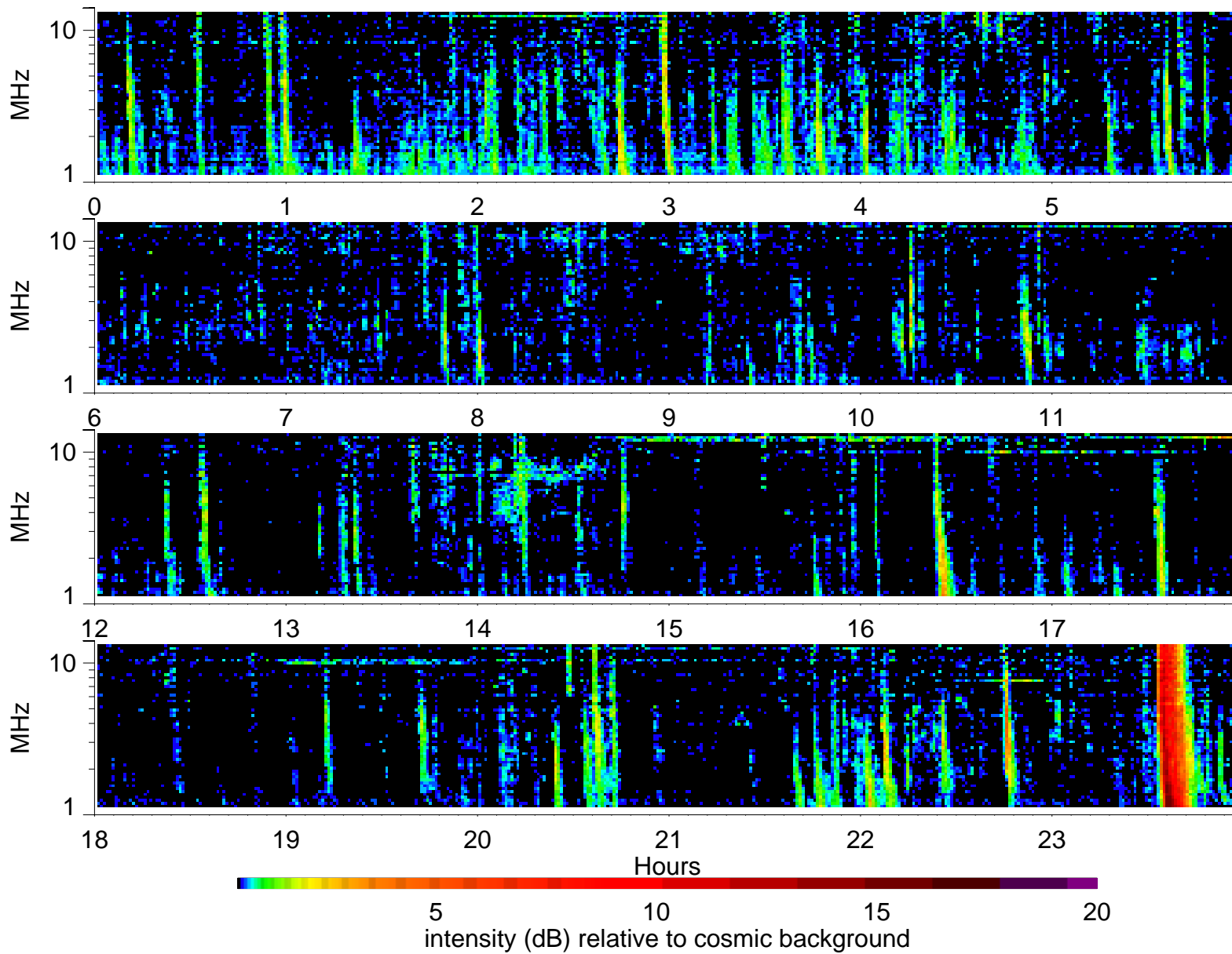
Wind Waves RAD2 receiver: 2005/2/16
