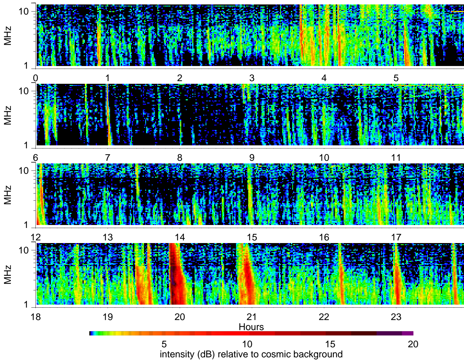
Wind Waves RAD2 receiver: 2005/2/14
