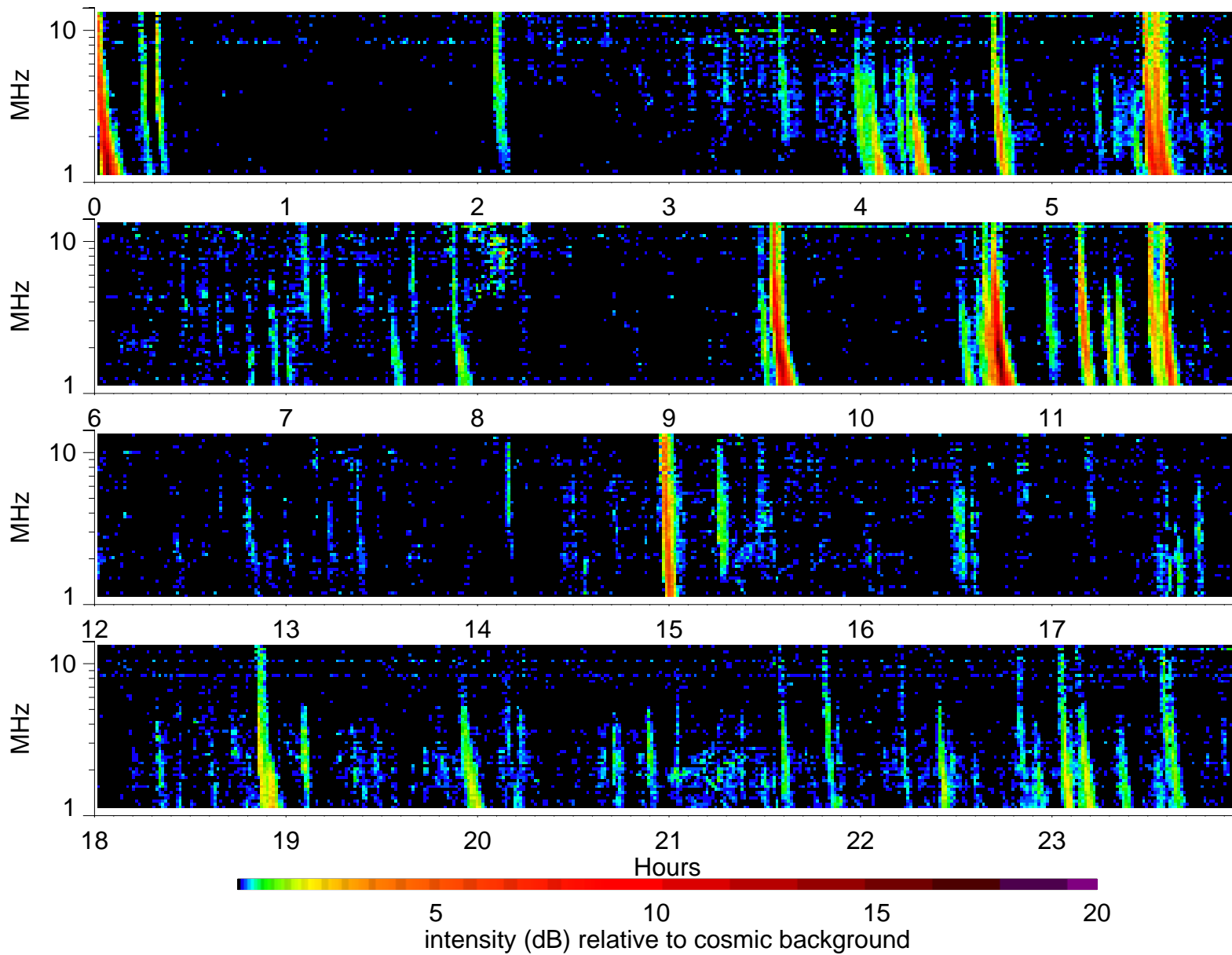
Wind Waves RAD2 receiver: 2005/2/10
