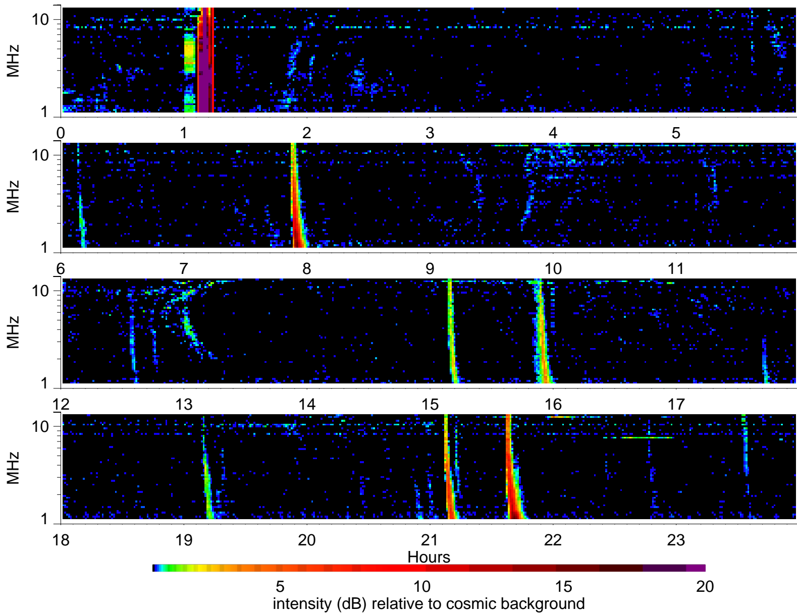
Wind Waves RAD2 receiver: 2005/2/9
