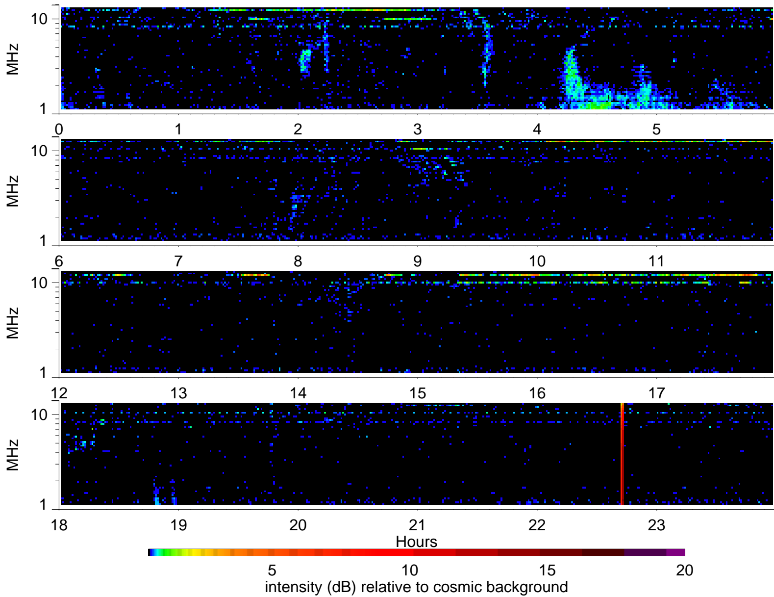
Wind Waves RAD2 receiver: 2005/2/6
