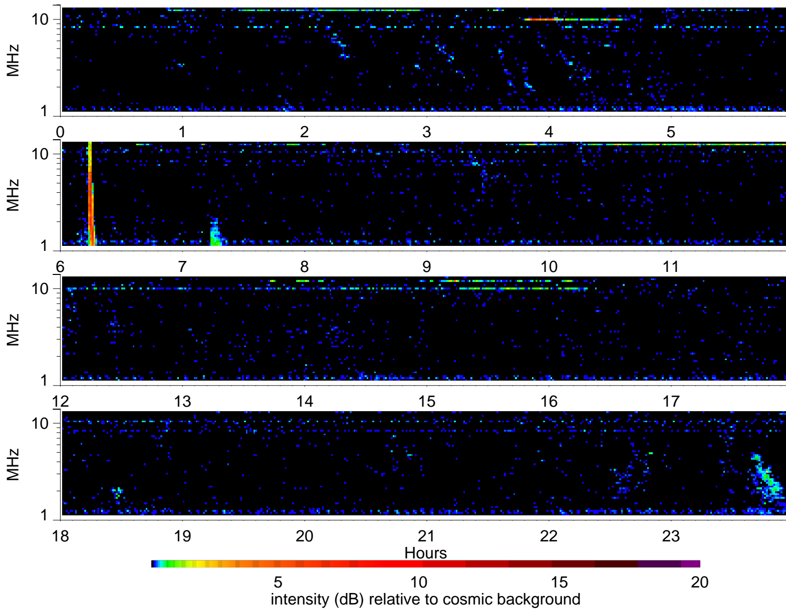
Wind Waves RAD2 receiver: 2005/1/31
