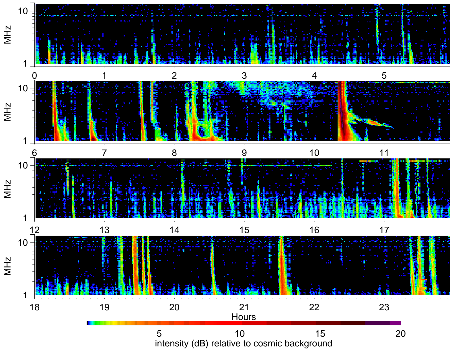
Wind Waves RAD2 receiver: 2005/1/19
