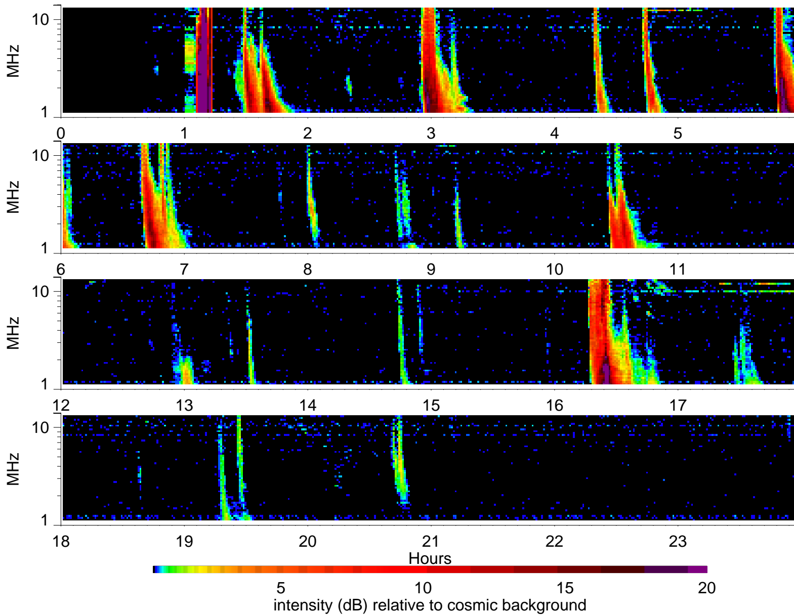
Wind Waves RAD2 receiver: 2004/12/29
