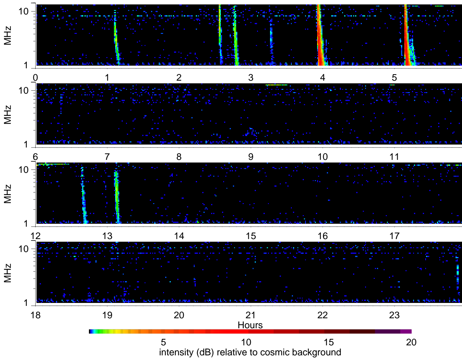
Wind Waves RAD2 receiver: 2004/12/26
