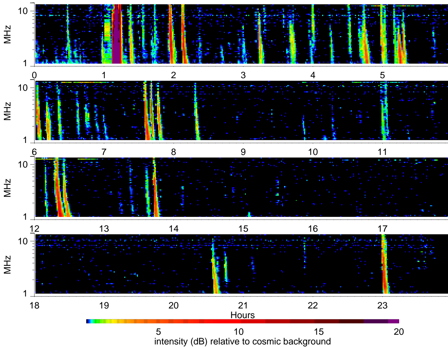
Wind Waves RAD2 receiver: 2004/12/23
