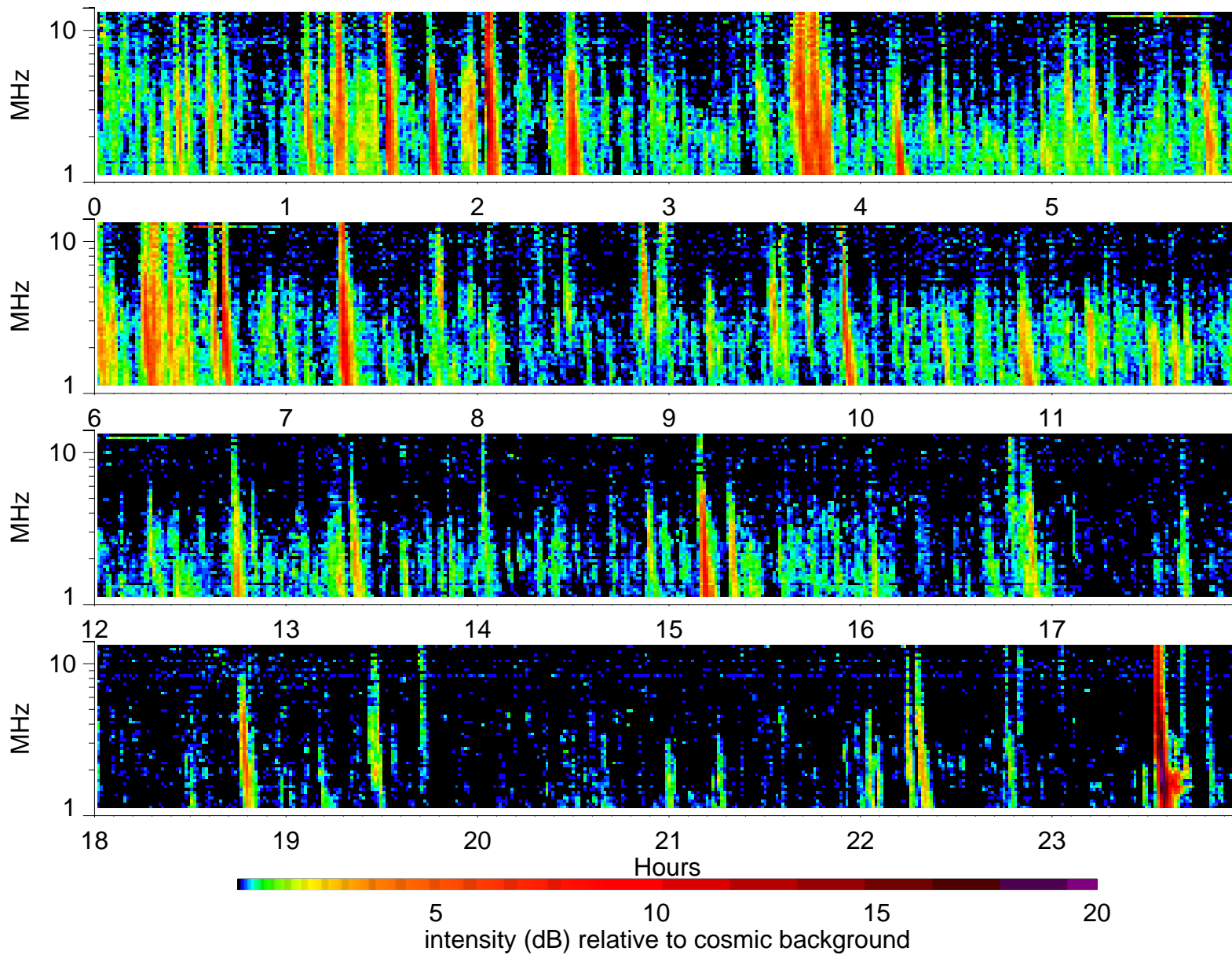
Wind Waves RAD2 receiver: 2004/12/22
