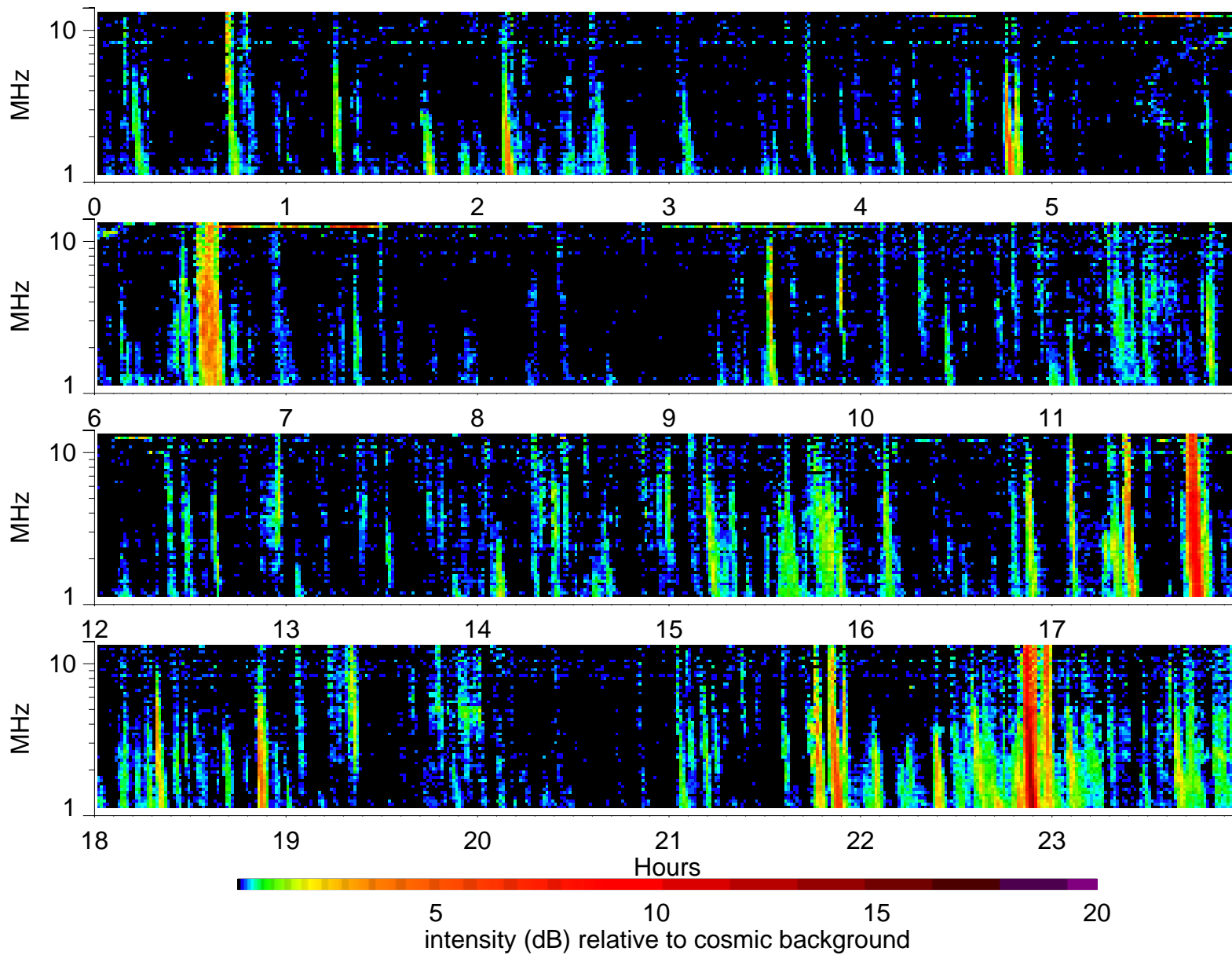
Wind Waves RAD2 receiver: 2004/12/20
