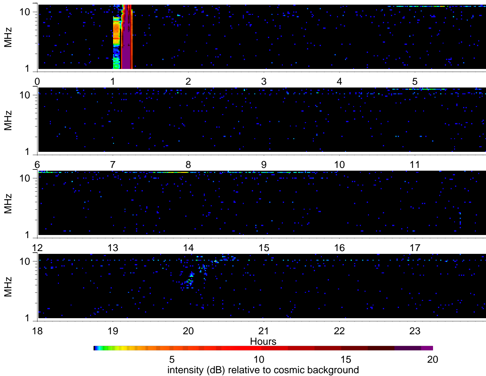
Wind Waves RAD2 receiver: 2004/12/7
