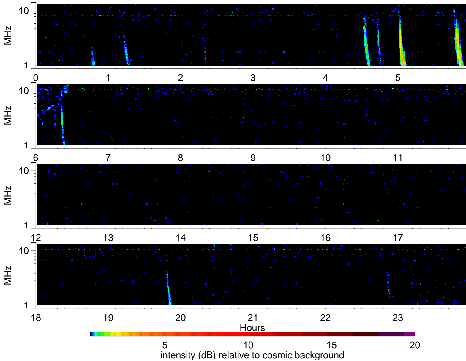
Wind Waves RAD2 receiver: 2004/11/26
