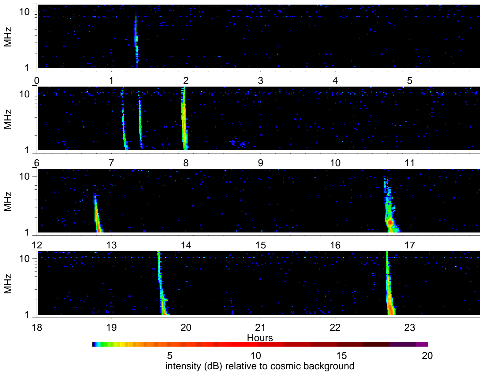
Wind Waves RAD2 receiver: 2004/11/24
