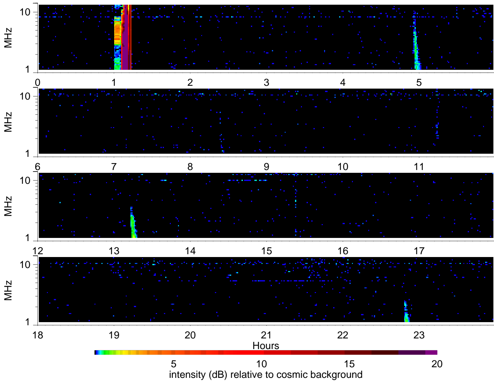
Wind Waves RAD2 receiver: 2004/11/21
