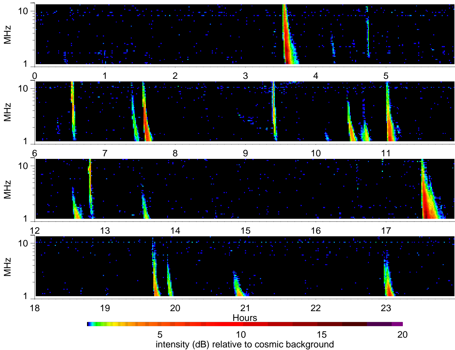
Wind Waves RAD2 receiver: 2004/11/18
