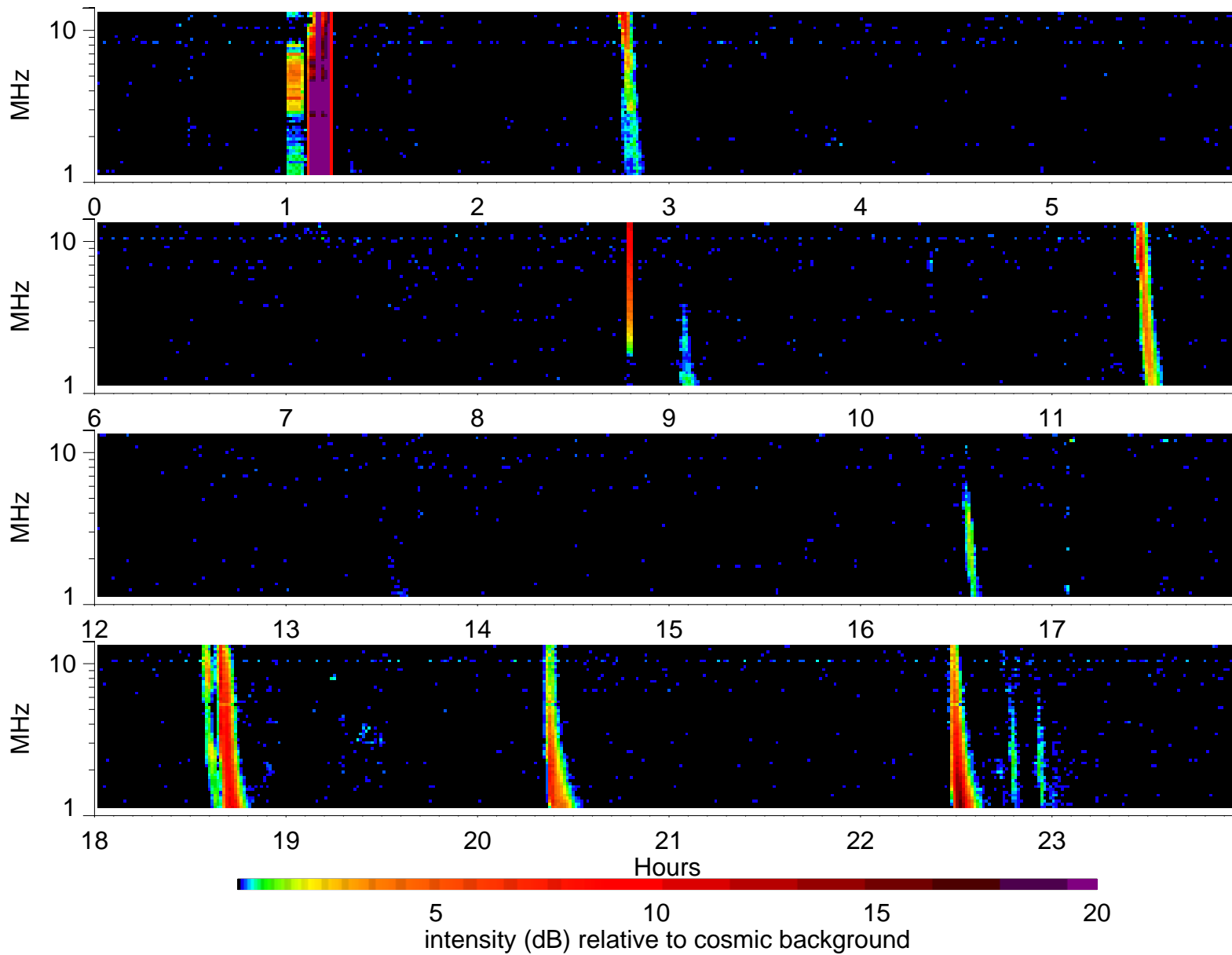
Wind Waves RAD2 receiver: 2004/11/17
