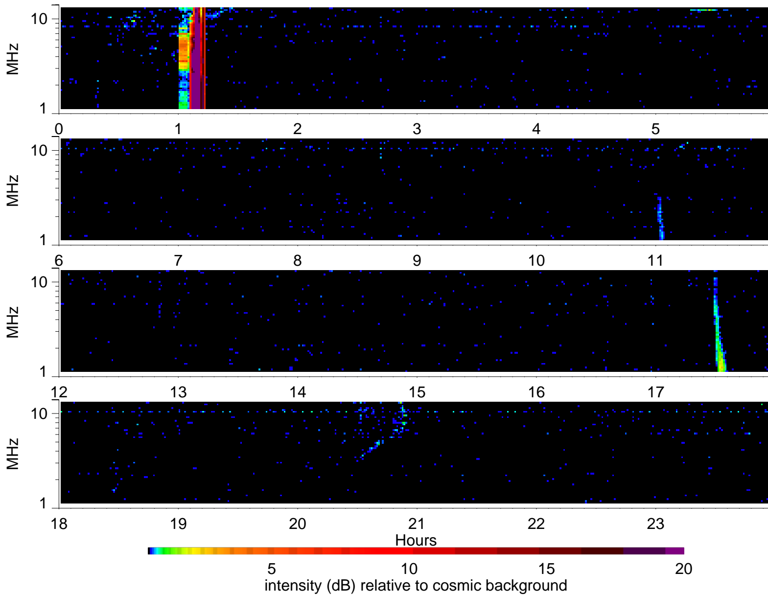
Wind Waves RAD2 receiver: 2004/11/13
