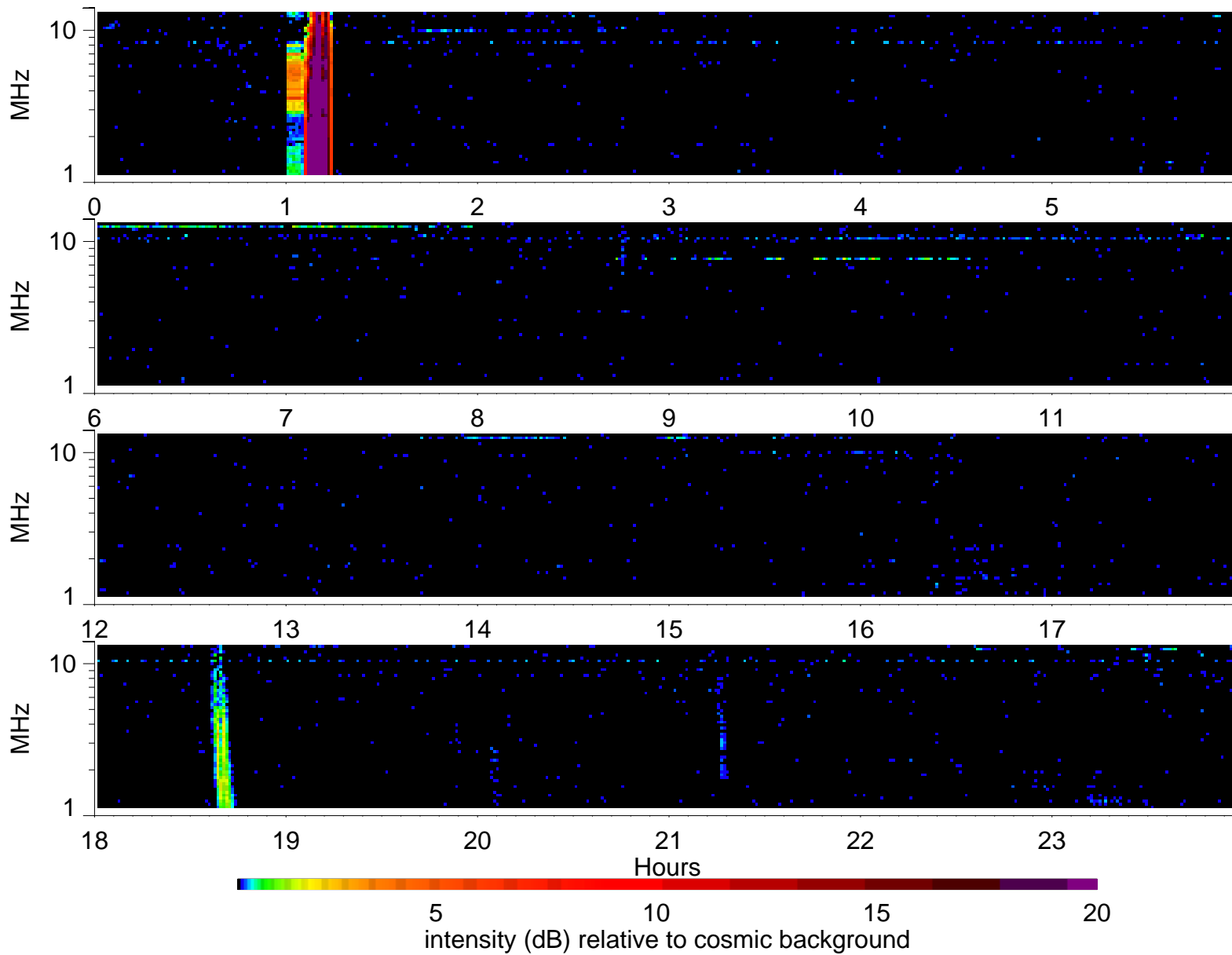
Wind Waves RAD2 receiver: 2004/11/11
