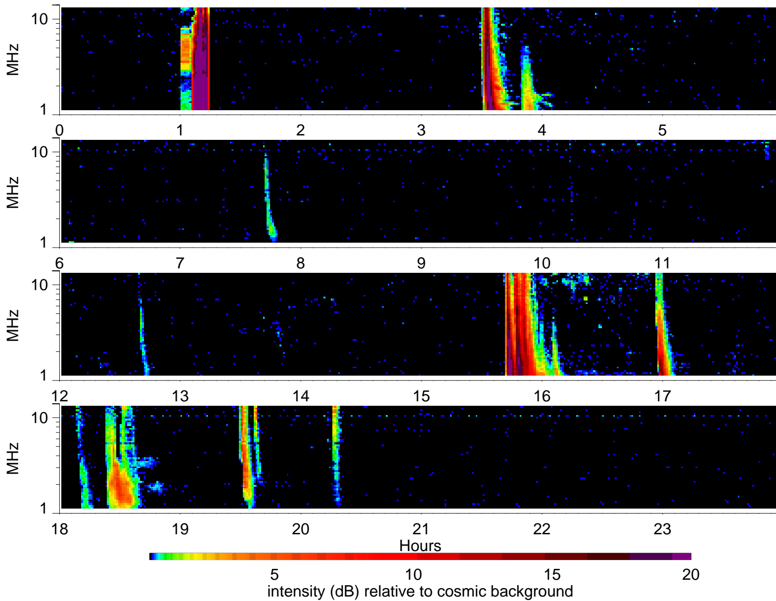
Wind Waves RAD2 receiver: 2004/11/3
