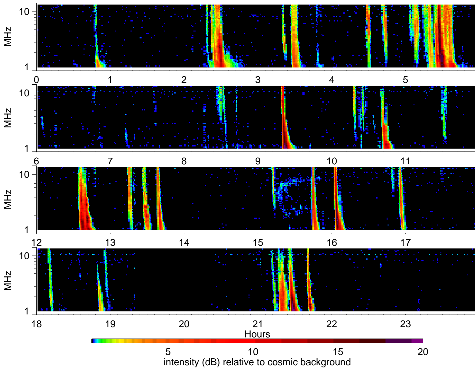
Wind Waves RAD2 receiver: 2004/10/31
