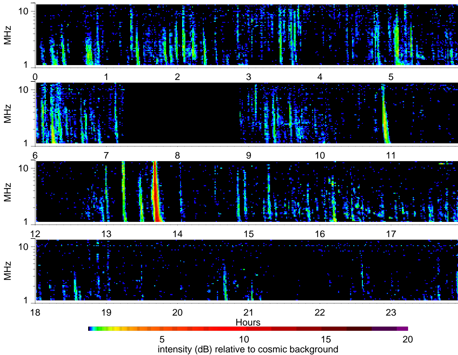
Wind Waves RAD2 receiver: 2004/10/27
