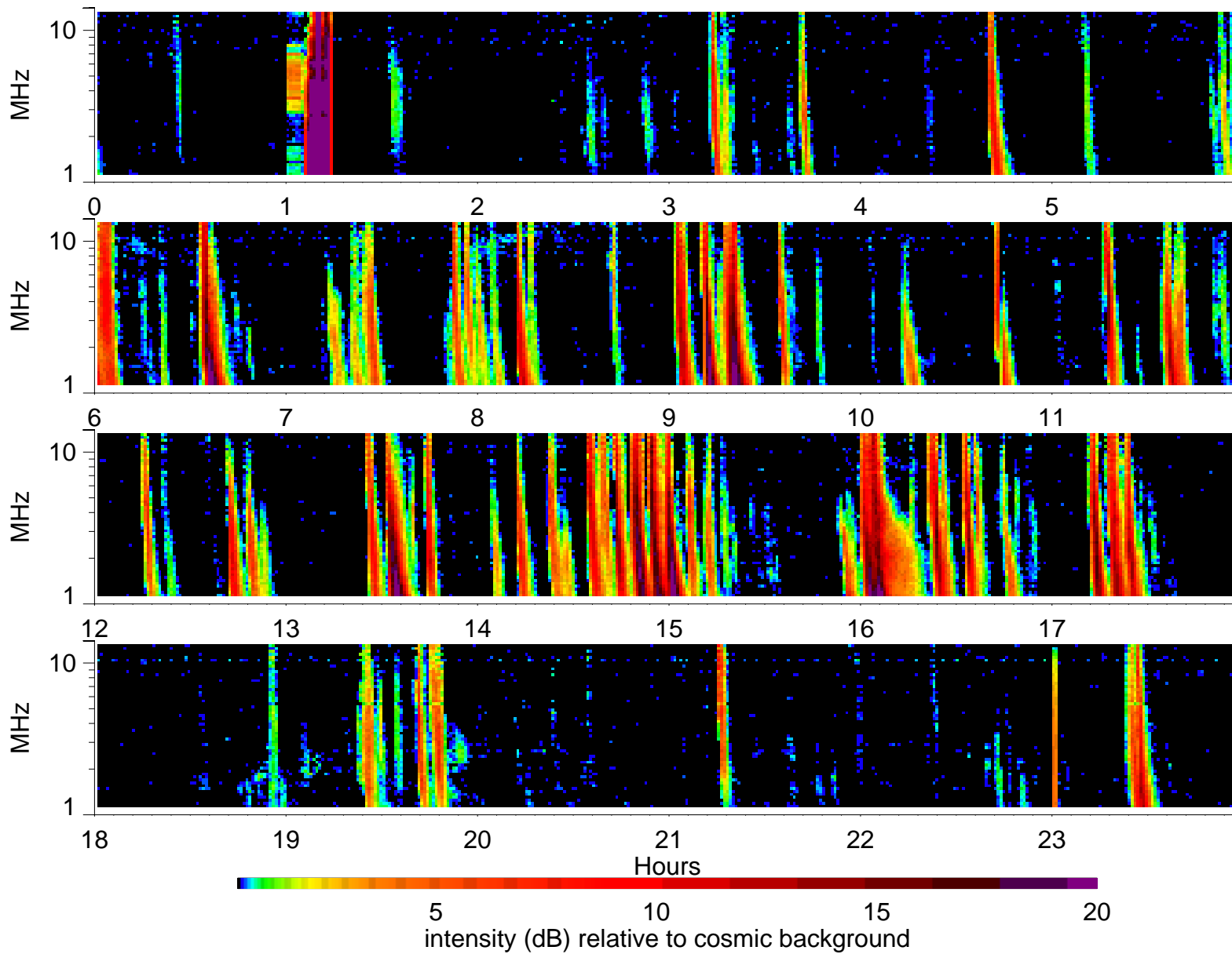
Wind Waves RAD2 receiver: 2004/10/26
